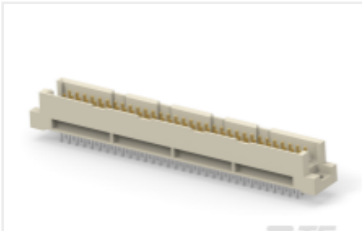
TE 产品编号374199-E STVR 96 MI ABC VVV 4-00 GA06 4,0 * 137 E
