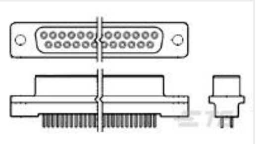
TE 产品编号5745080-6 HD-20 RCPT 50P VERT FFSCRLK
