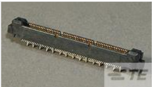
TE 产品编号 1-5767149-0 MICTOR PLUG ASSY IN TAPE & REE
