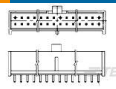
TE 产品编号5-1658549-3 FPH-6022G=FLXPAC HDR P ST LF
