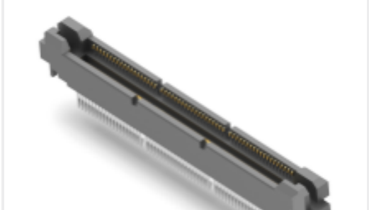
TE 产品编号 5767039-3 MICTOR,RA PLUG,114,.093PCB,ASY
