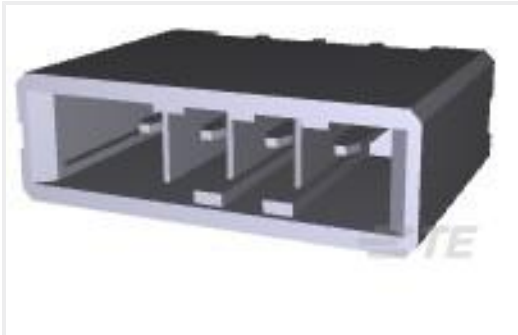
TE 产品编号2-917338-3 DYNAMIC 3200 VERTI. HDR ASY 4P
