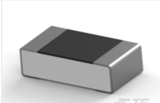
TE 产品编号2-2176370-6 RQ 0603 787R 0.1% 10PPM 5K RL
