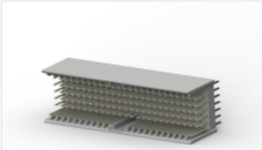
TE 产品编号5646529-1 Z-PACK 2MM HM TYPE A/B 169P
