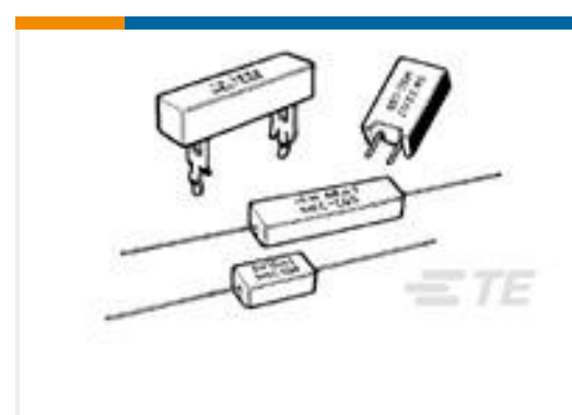
TE 产品编号1623788-8 SQM5 18R 5% (WIRE)
