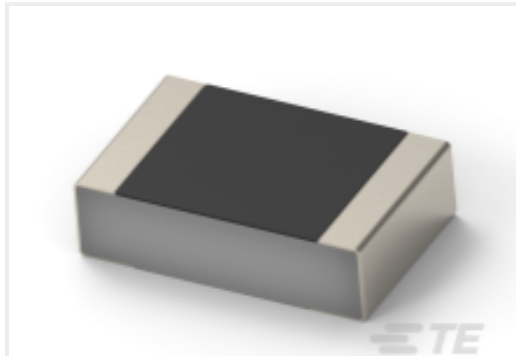
TE 产品编号4-2176451-0 CPF 0201 127R 0.1% 25ppm 1K RL
