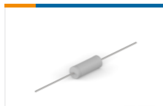
TE 产品编号5-2176412-8 5W XSM M/OX 5% 1K2
