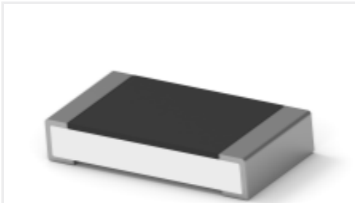
TE 产品编号6-2176389-5 RQ 1206 499R 0.1% 10PPM 5K RL
