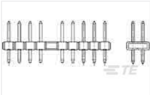
TE 产品编号5176264-4 AMPMODU 2MM V 10P AU:0.2 BLACK LF
