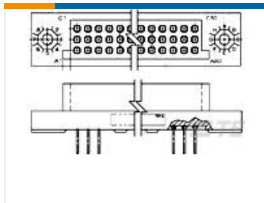
TE 产品编号531134-1 3ROW BOX REC 90P 100CL UNSEAL
