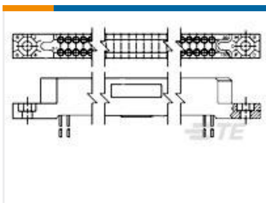
TE 产品编号531142-9 2 ROW BOX RECP 90 POS STAG
