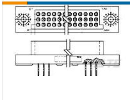
TE 产品编号531134-3 3ROW BOX REC 120P 100CL UNSEAL
