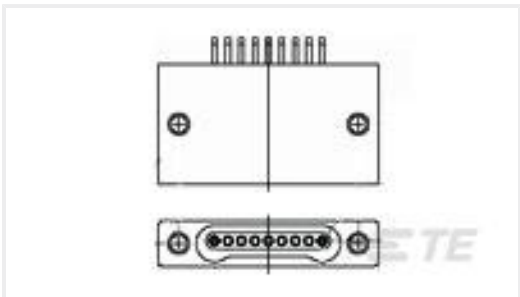
TE 产品编号4-1589462-3 SSM051L2AQ = SMT CONN
