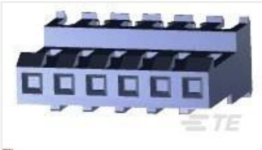
TE 产品编号3-640601-6 06P MTA156 CONN ASSY 22AWG LF
