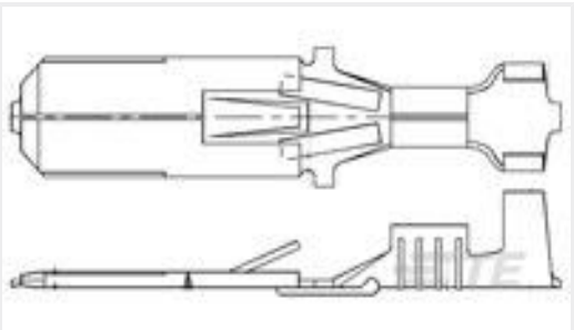
TE 产品编号160451-2 FF 250 TAB 18-14AWG TPPB LP
