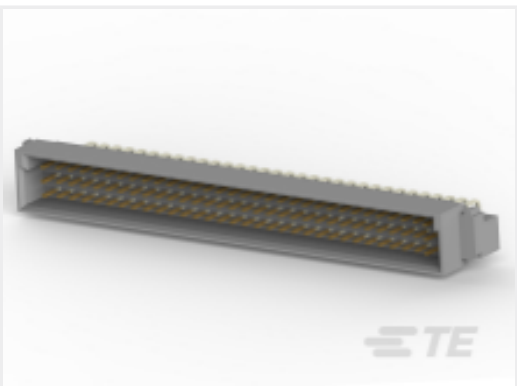
TE 产品编号 5536437-4 ASSY,PIN,EUROCARD,TYPE C,LEAD-OUT,FREE,96 PO
