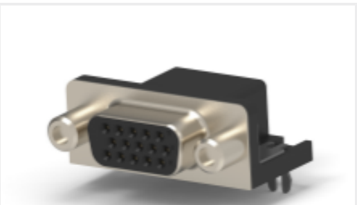
TE 产品编号2311763-1 AMPL REC, HD22, R/A, 15P, S/L
