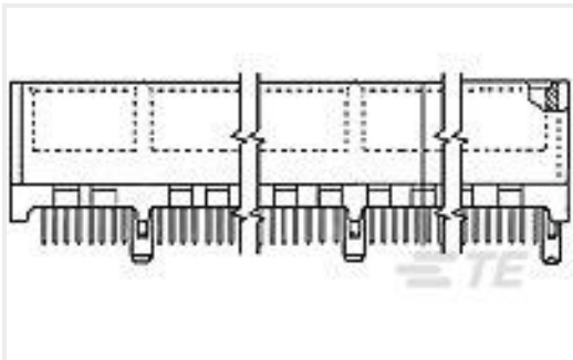
TE 产品编号5145165-4 STANDARD EDGE .050 SERIES 92 DUAL ASSY
