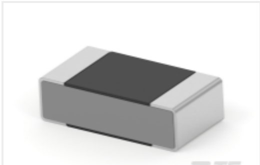
TE 产品编号7-1879417-0 CPF0603 634K 0.1% 25PPM 1K RL
