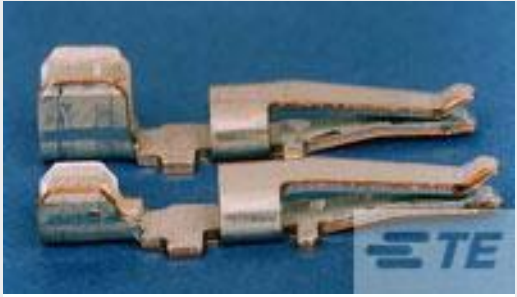
TE 产品编号556136-2 CONT,AMPINNERGY WTW,LS PC,10-12
