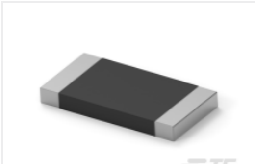
TE 产品编号5-2176421-3 TLRP 2512 2.0W R020 1% 50PPM 4K RL
