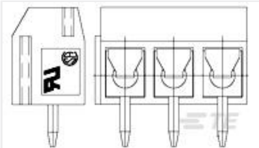
TE 产品编号1776266-3 3P TB ,90deg, VT, 5mm,Green,w /interlock
