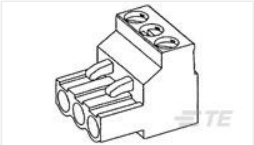
TE 产品编号796635-3 3 POS 5.08MM R/A PLUG,TRM BLK
