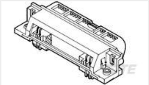
TE 产品编号5552791-1 ASSY, RCPT, 24 POSN, RTANG PCB
