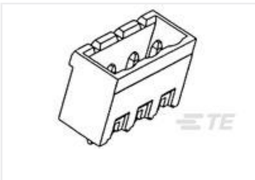
TE 产品编号796637-3 3POS 5.08MM CE VRT HDR,TRM BLK
