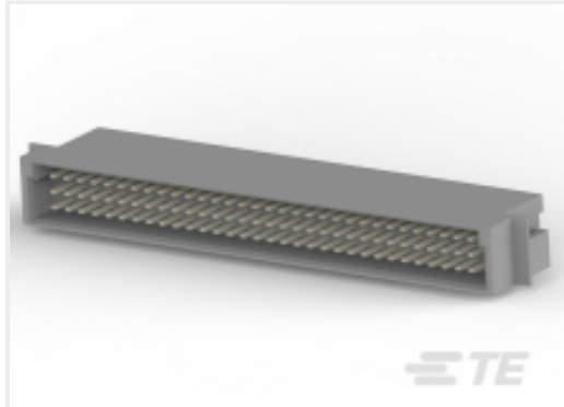
TE 产品编号 215605-4 96P.IEC-C MALE CONN
