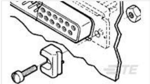
TE 产品编号747080-2 LATCH BLOCK/PACKAGED/.090 PANL
