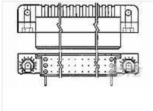
TE 产品编号5533268-5 ASSY,RECPT,R.ANGLE,HDI,LEAD-FR
