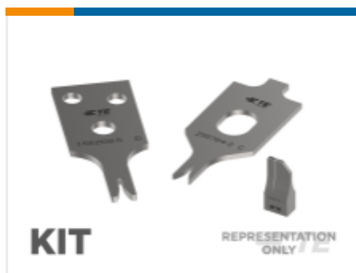
TE 产品编号7-2837297-7 OCEAN_2.0_SPARE_PART_KIT-042F055O
