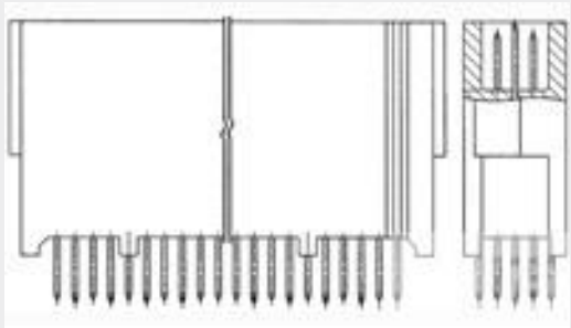
TE 产品编号5536272-9 200,PLUG,VT,125,30AU
