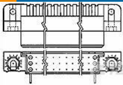
TE 产品编号533268-1 HDI RECP ASSY 3 ROW 75 POS
