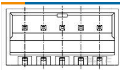
TE 产品编号5-1775444-3 EMIX CONN., 1.5MM PITCH, HDR, R /A, 3P
