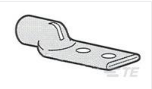
TE 产品编号326803 TERM, AMPOWER, 4/0, 3/8, 2 HOLE
