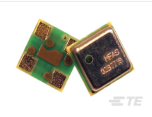
TE 产品编号MS563702BA03-50 2 BAR INDUSTRIAL ALTIMETER SENSOR
