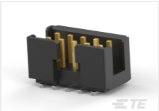
TE 产品编号1-2373376-0 10P,2MM,SHRD HDR,DRV, SMD,0.1 AU,TB
