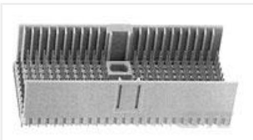
TE 产品编号1-2000713-0 RA Keyed Guide Mod, Vita 46, Machined
