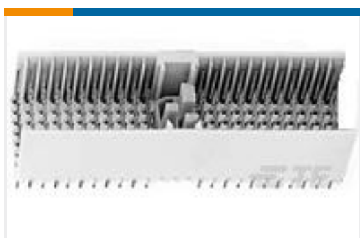
TE 产品编号5188399-1 TYPE A, FIXED BOARD M /CONNECTOR
