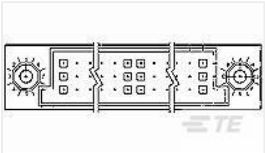
TE 产品编号532447-9 HDI PIN ASSY 3 ROW 180 POS
