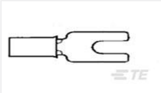
TE 产品编号2-327735-1 PG SPD 22-16 COMM 22-18 MIL 6
