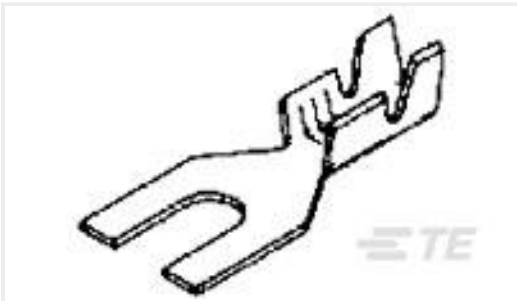
TE 产品编号60773-2 SPADE TERMINAL 18-14 AWG TPBR
