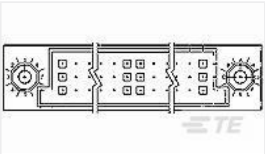
TE 产品编号 650841-1 HDI PIN ASSY 3ROW 165/107 POS
