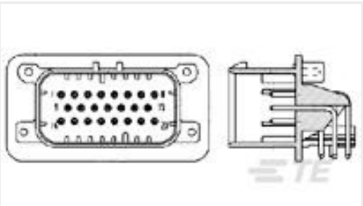
TE 产品编号770669-1 23POS,PIN DIA 1.3,HDR ASSY,90DEG, COD 1
