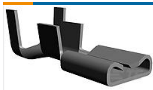
TE 产品编号42660-2 250 FASTON REC 18-14 AWG TPBR
