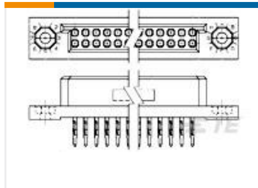
TE 产品编号5-533289-5 BOX II 2 ROW RECP ASSY 60 POS
