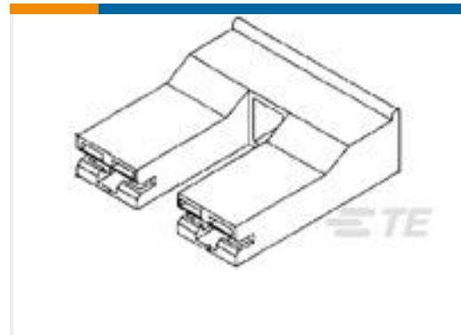
TE 产品编号521119-1 PL 250 HOUSING RECEPTACLE NYLON 6/6
