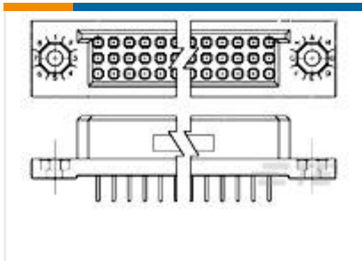
TE 产品编号533287-4 BOX II ASSY 105 POS W/SOLD TL
