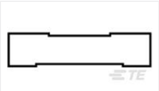
TE 产品编号55792-2 PG BUTT SPLC 22-16COMM22-18MIL
