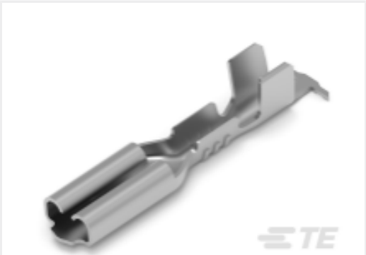
TE 产品编号2238095-1 110 FASTON,REC.,22-20 AWG,PTBR
