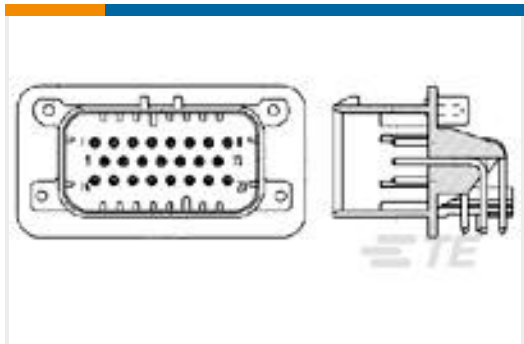
TE 产品编号776087-1 23POS,PIN DIA 1.3,HDR ASSY,90DEG, COD 1
