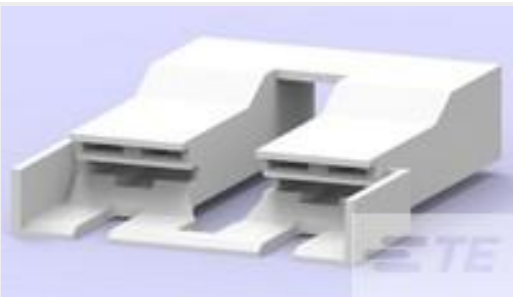
TE 产品编号521253-2 PL 250 HSG REC RED NYLON 6/6
