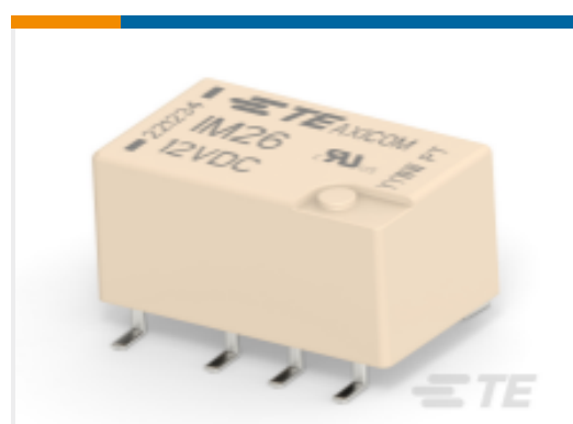
TE 产品编号3-1462039-1 IM26GR=IM RELAY 50mW 12V
